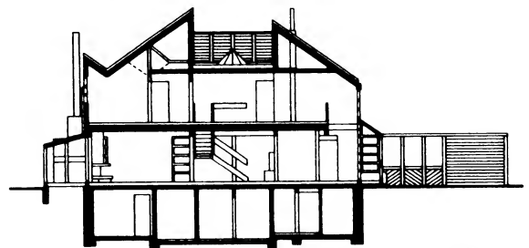
13 Section
